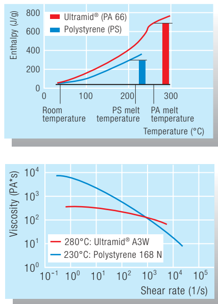
Figure 11: Enthalpy, viscosity and melt- ing profiles for two different materials
