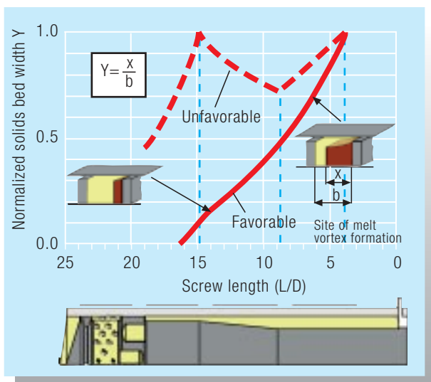
Figure 9: Comparison of different melting profiles
