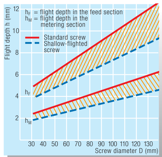
Figure 2: Flight depths for three-section screws
