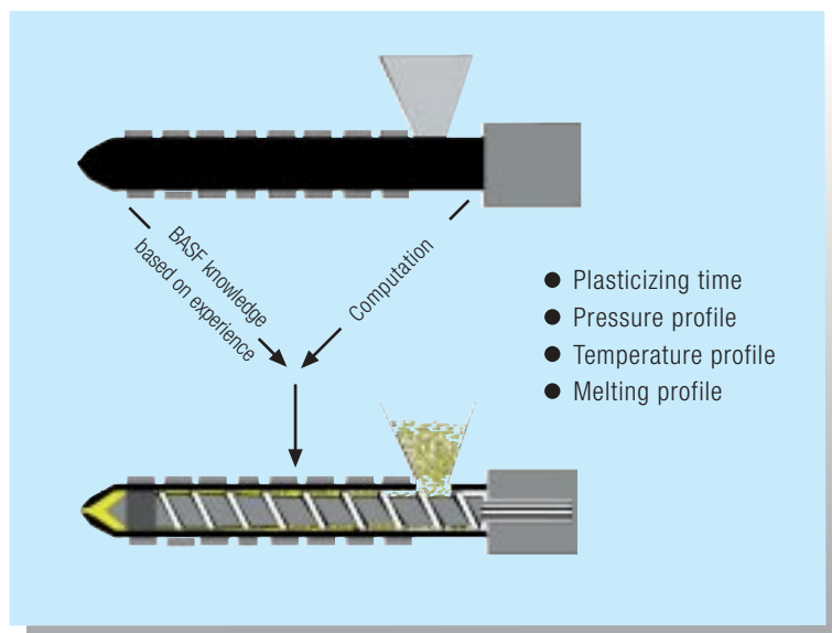
Figure 8: More predictable plasticating units as a result of simulation
