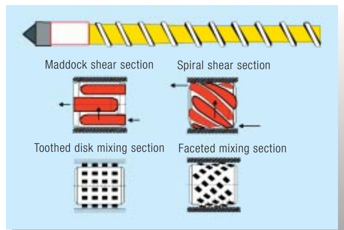
Figure 4: Three-section screw with commonly used shear and mixing sections
