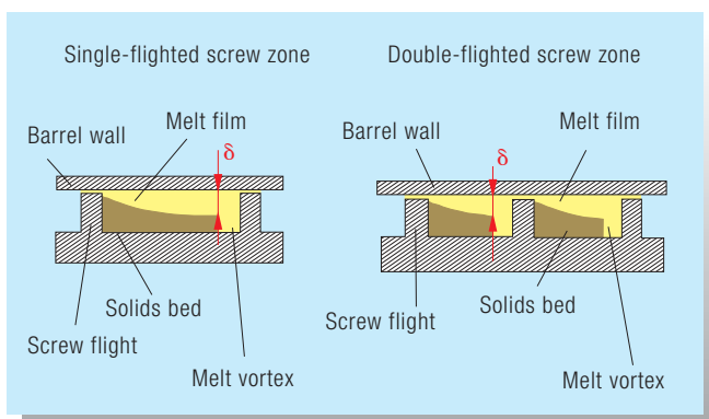
Figure 5: Section through the melting section of a single-flighted and a double-flighted screw
