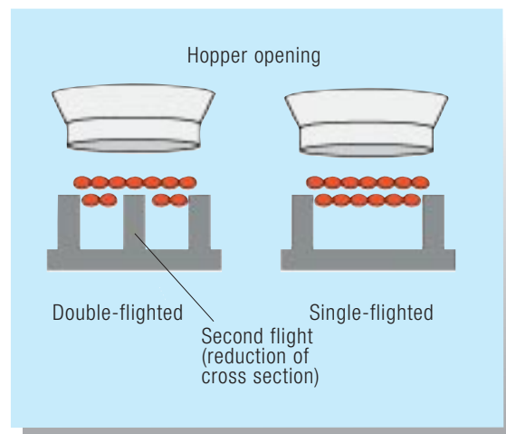
Figure 6: Charging cross sections in single-flighted and double-flighted screws
