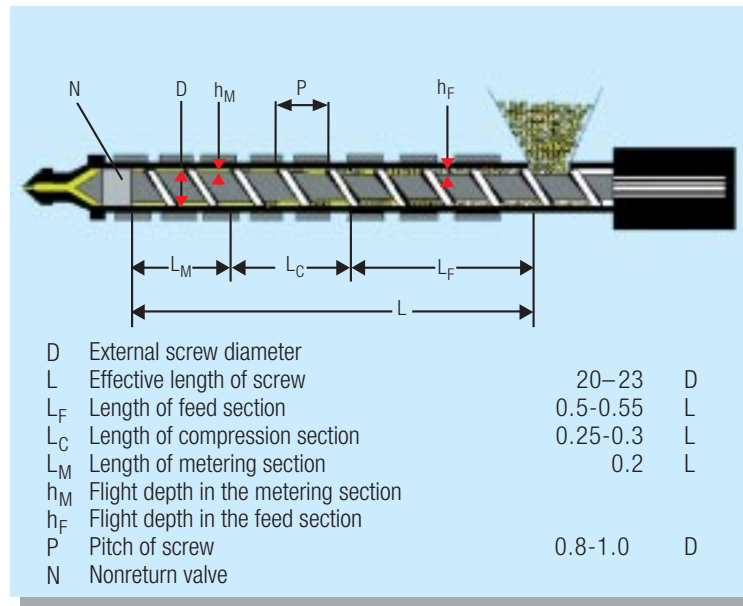
Figure 1: Plasticating unit with a three-section screw
