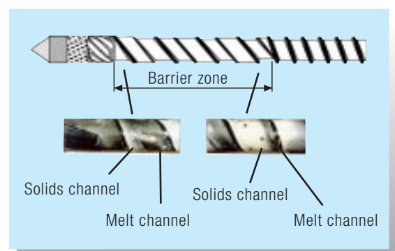
Figure 10: Barrier zone with closed inlets and outlets
