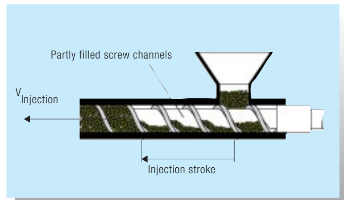
Figure 3: Trickle feed of material during injection
