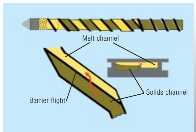
Figure 7: Principle of a barrier screw
