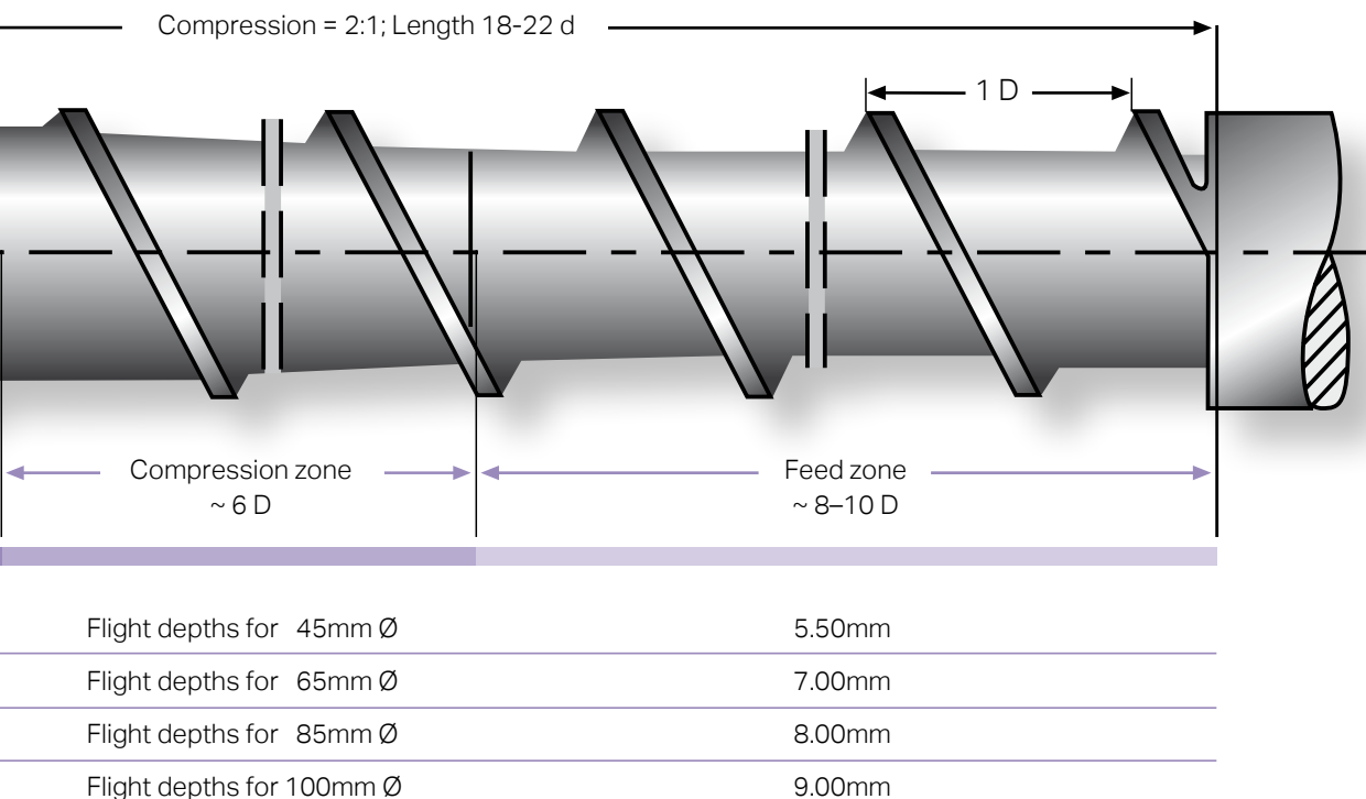
Injection molding screw for processing Covestro’s TPU
