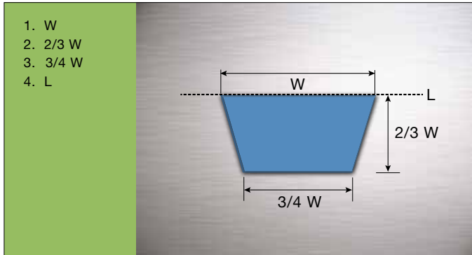
Figure 1: Relative Dimensions of a Trapezoidal Runner for Use in a Three-plate Mold
