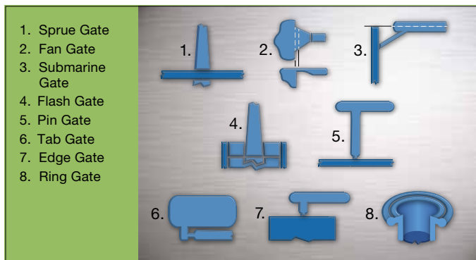
Figure 4: Gate Designs
