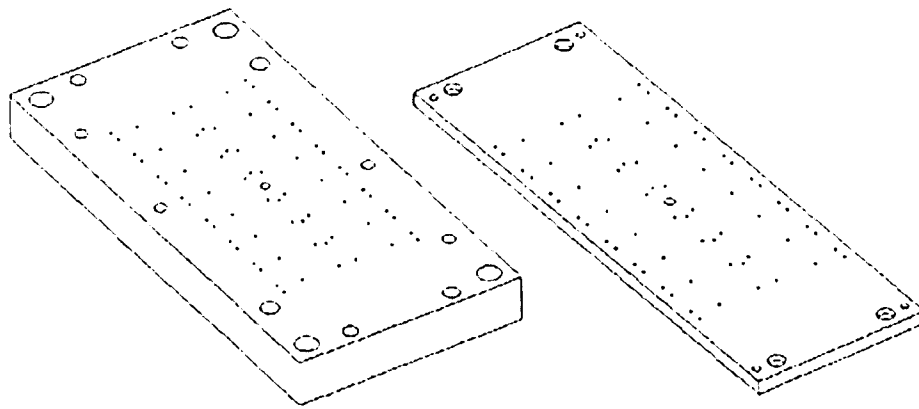
Figures 3-13: The Support and Ejector Retainer Plates
