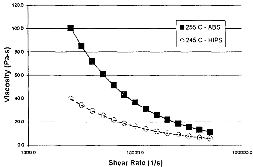
Figure 5-10: Viscosity Plot for ABS and HIPS at Operating Temperature
