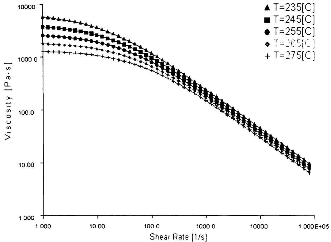
Figure 5-9: Viscosity vs Shear Rate Plot for DOW 1040 ABS
