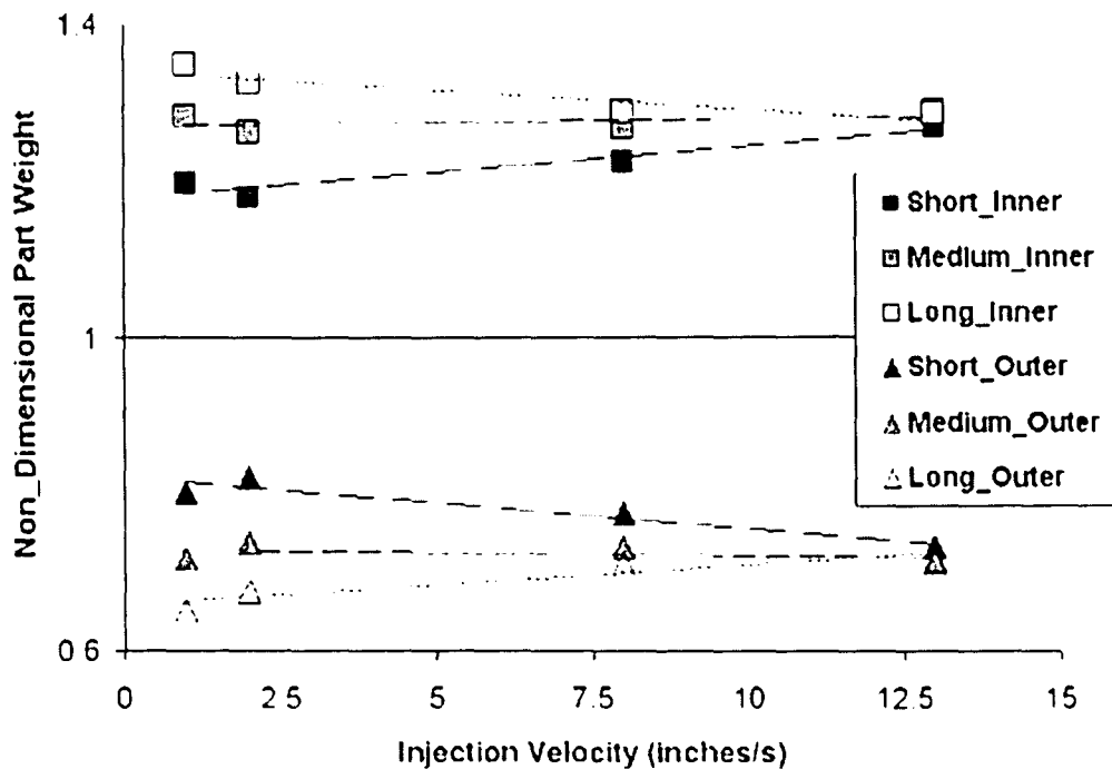
Figure 5-3: Fill Imbalance with respect to Injection Velocity (ABS)
