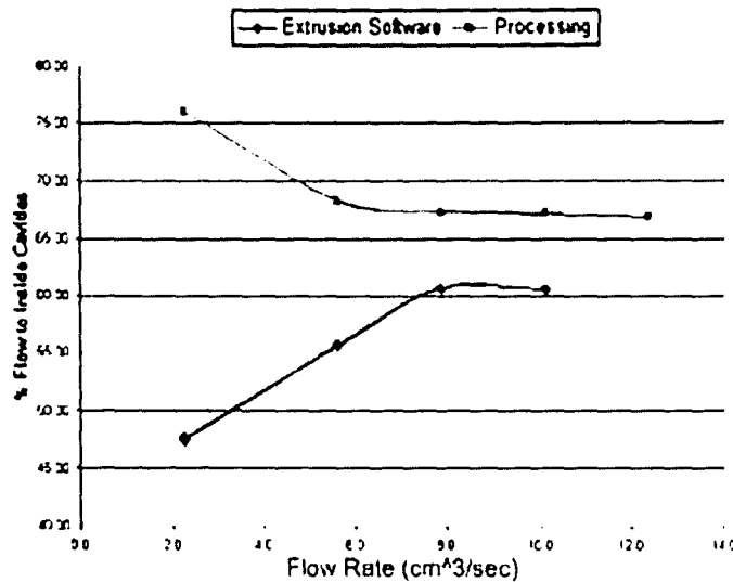
Figure 2-18: Simulation vs Actual Results [12]
