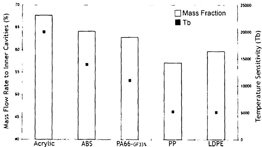
Figure 2-20: Viscosity Temperature Sensitivity factor versus Fill Imbalance [1]
