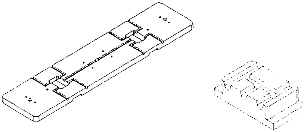
Figures 3-7: Medium Runner Bar & Runner Intersection Insert
