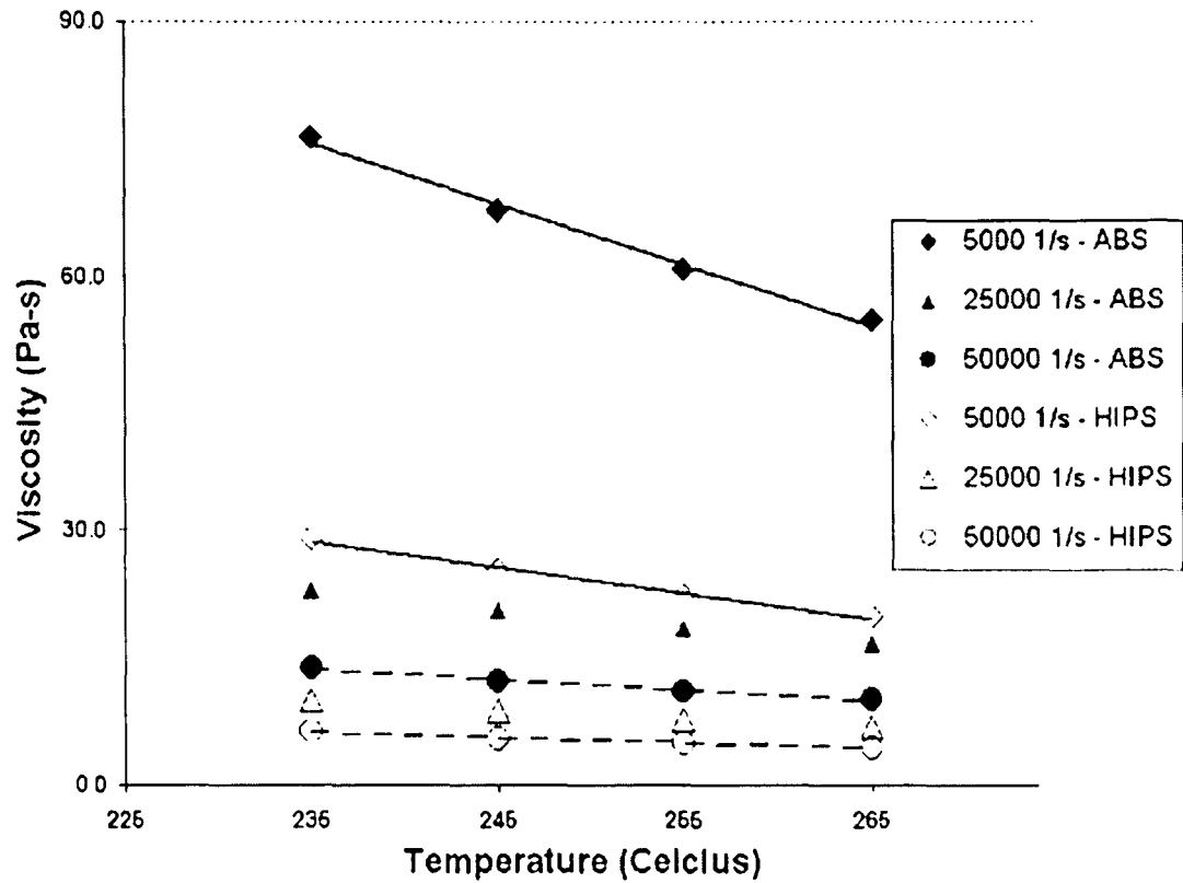
Figure 5-11: Viscosity Relative to Temperature and Shear Rate
