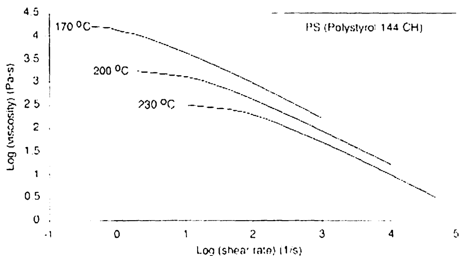
Figure 2-7: A Polymer Viscosity's Relationship to Shear Rates [8]
