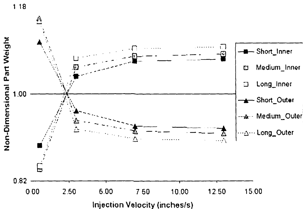
Figure 5-6: Fill Imbalance with respect to Injection Velocity (HDPE)
