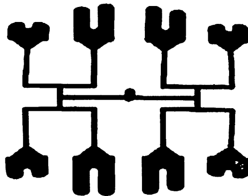
Figure 1-1: Fill Imbalance in Geometrically Symmetrical Runner Mold
