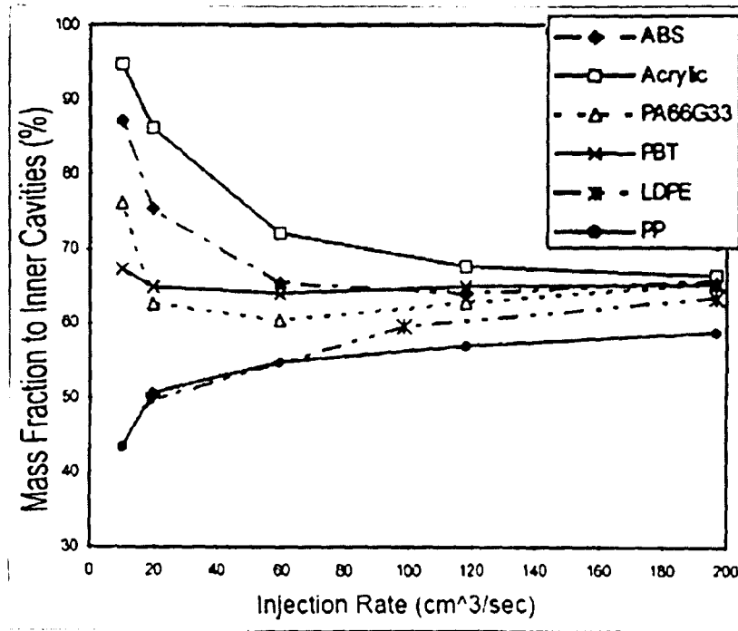
Figure 2-19: Fill Imbalance Dependence to Polymer Material [1]
