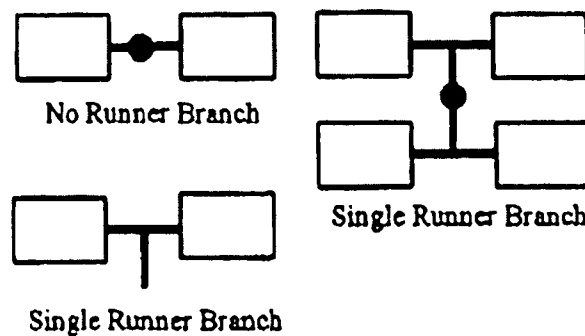
Figure 2-9: Naturally Balanced Molds with less than 8 Cavities
