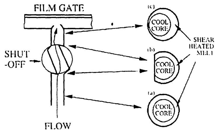
Figure 2-23: Effect of Runner Geometry Changes on Melt Domains [14]
