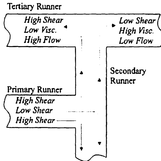
Figure 2-12: Second Separation of Melt Laminates [1]
