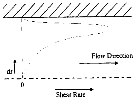
Figure 2-8: Shear Rate Profile Across a Circular Runner [1]
