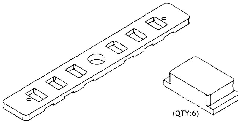
Figure 3-11: A-Half Retainer Plate & Blank Insert
