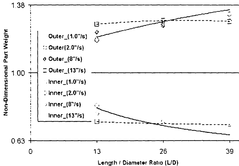
Figure 5-4: Fill Imbalance with respect to L/D Ratio (ABS)
