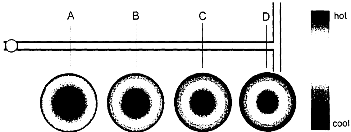
Figure 5-8: Shift of Temperature Profile with Distance for Reverse Fill Imbalance
