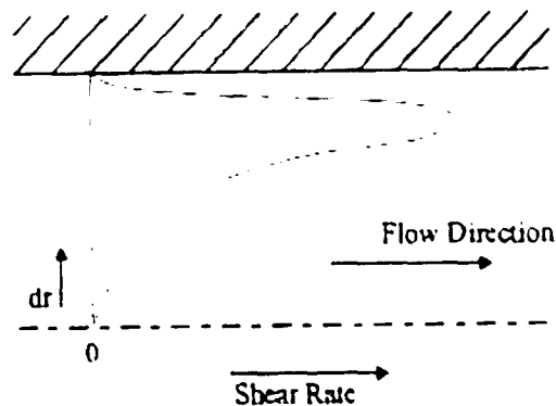
Figure 2-6: Shear Rate Profile in Circular Channel
