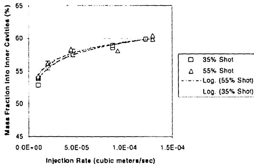
Figure 2-13: Fill Imbalance with respect to Injection Rate using PA-66 [10]
