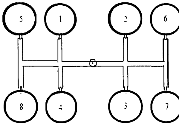
Figure 2-1: Early Design of Multi-Cavity Runner System
