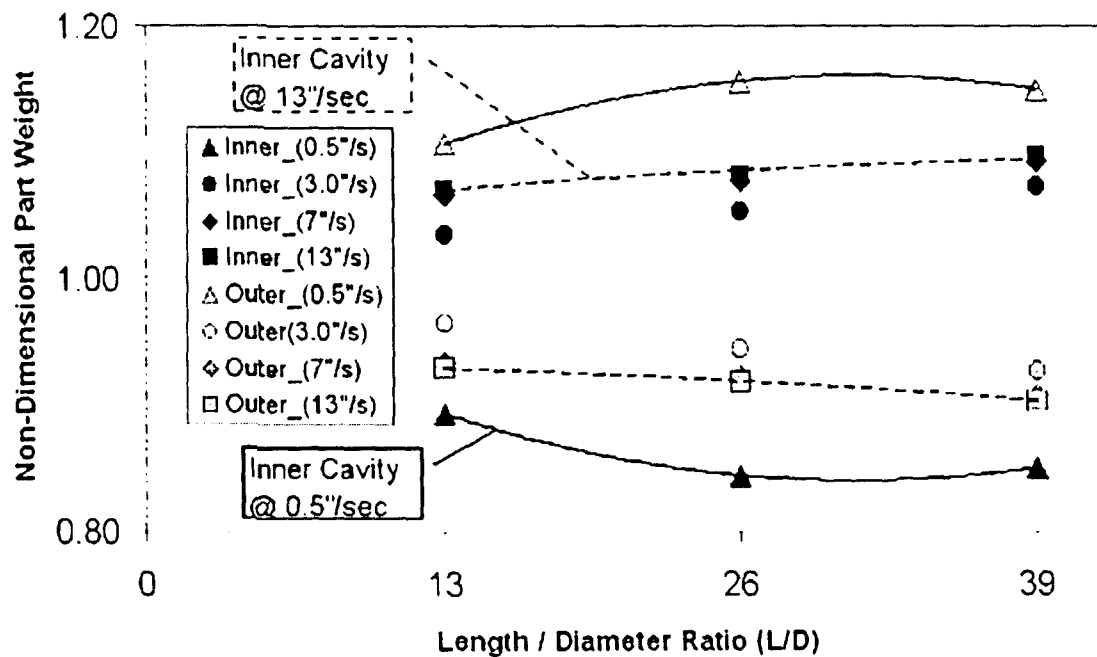
Figure 5-7: Fill Imbalance with respect to L/D Ratio (HDPE)
