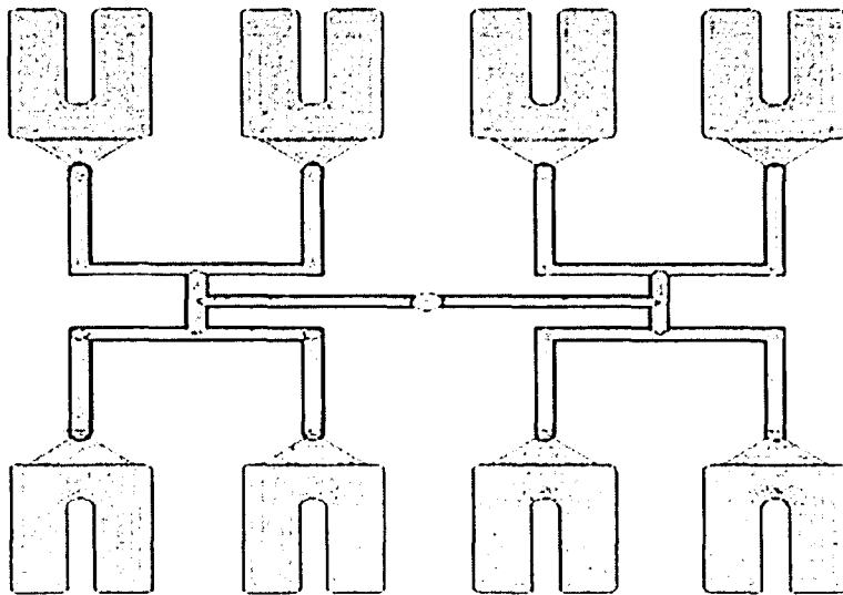
Figure 3-1: Base Design of Multi-Cavity Mold
