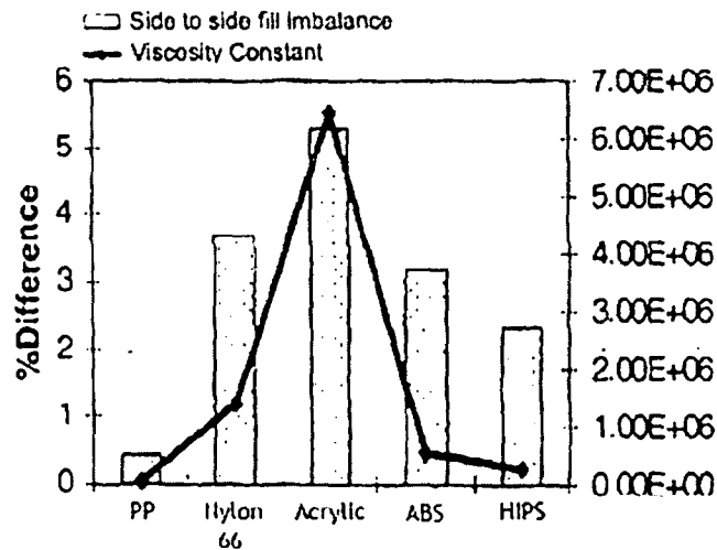
Figure 2-21: Side-to-Side Fill Imbalance Correlates with Viscosity Constant [13]
