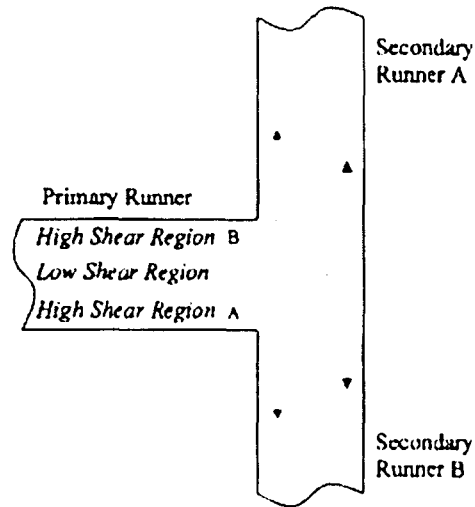
Figure 2-10: Initial Separation of Melt Laminates [1]
