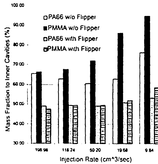
Figure 2-27: Comparison of Fill Imbalance with and without MeltFlipper™ [1]
