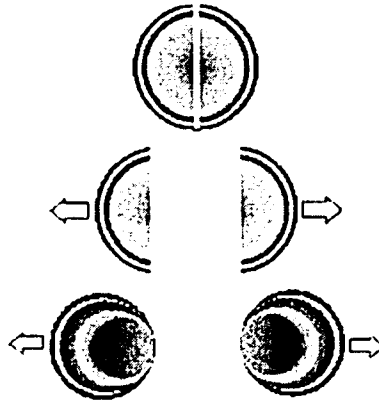
Figure 2-11: Imbalance of Viscosity / Temperature Profile [9]
