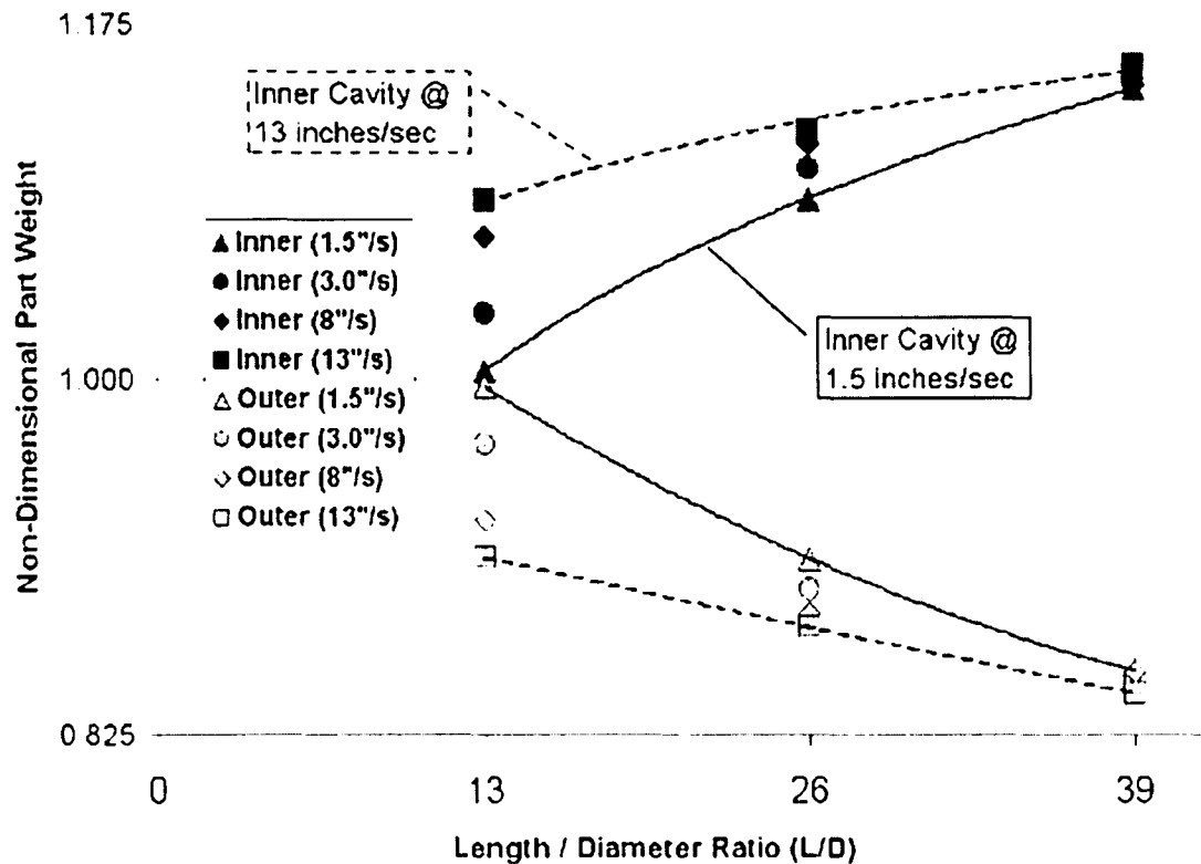
Figure 5-2: Fill Imbalance with respect to L/D Ratio (HIPS)
