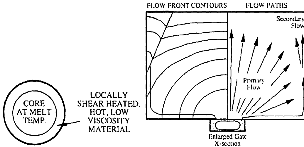
Figure 2-22: Shearing in Runner Causes Development of Secondary Flow [14]
