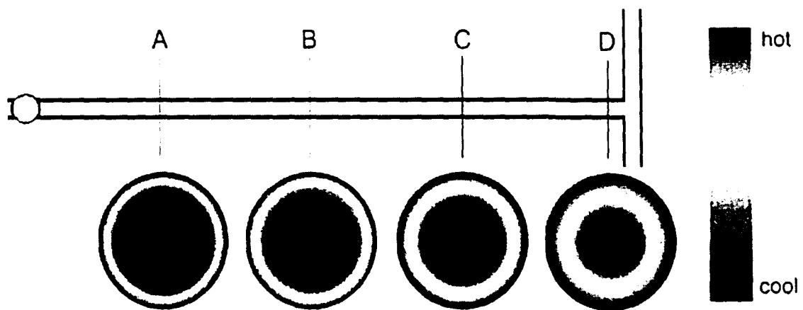
Figure 5-5: Shift of Temperature Profile with Increase of Runner Length
