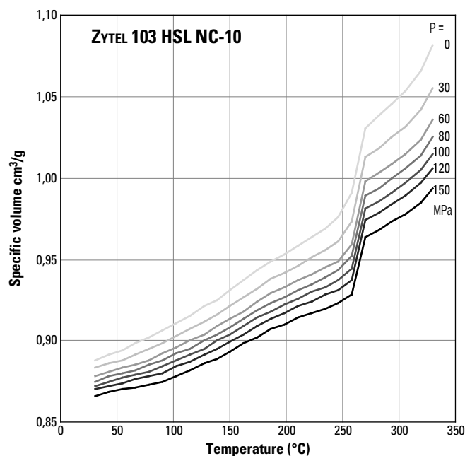
Fig. 1 Pressure-Volume-Temperature diagram (specific volume as a function of temperature and pressure)
