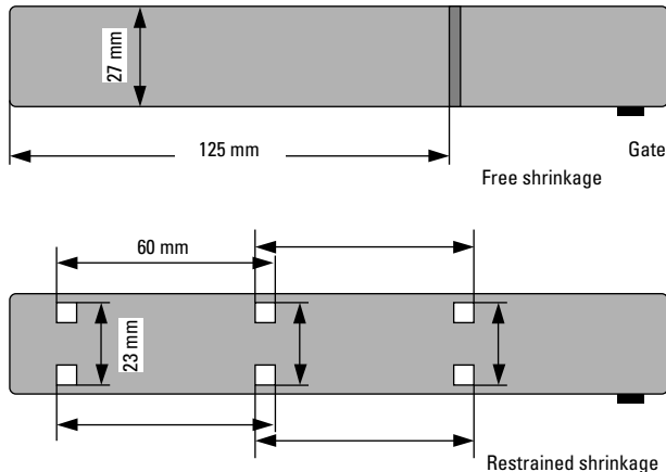
Fig. 53 Free vs. restrained shrinkage
