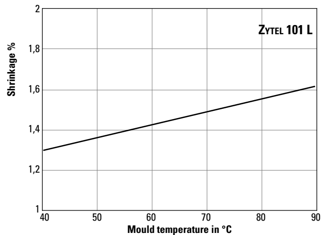
Fig. 49 Shrinkage as a function of mould temperature for a part 3 mm thick and a pressure of 90 MPa
