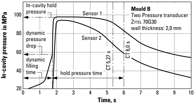
Fig. 10 Cavity pressure measured during the filling and packing (2 sensors)
