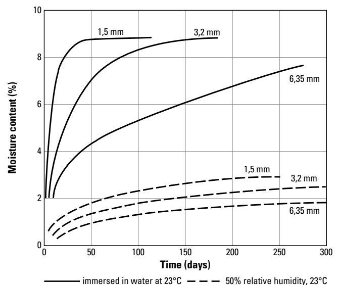
Fig. 55 Moisture contents as a function of time for moulded parts
