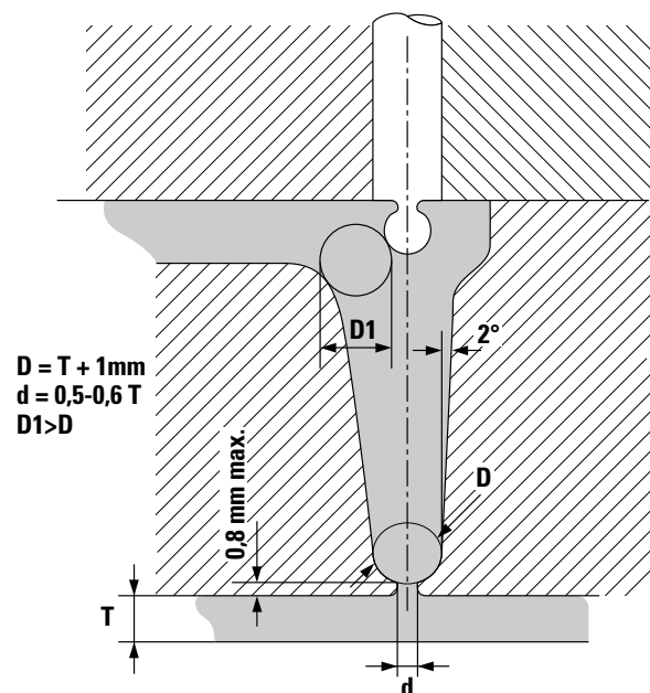
Fig. 23 Pin point gate design
