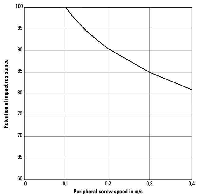
Fig. 47 Effect of screw speed on impact properties
