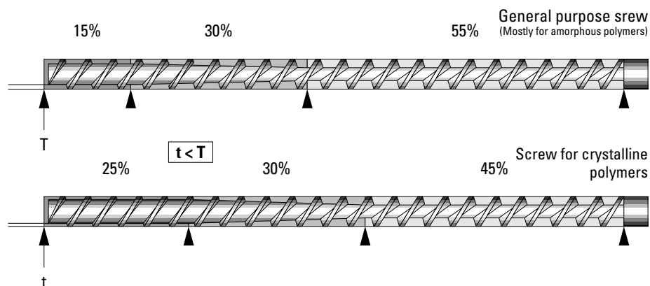
Fig. 19 Comparison of screw design
