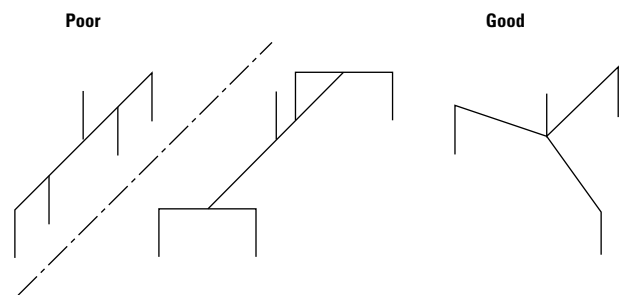
Fig. 32 Nozzle arrangement for multiple cavity mould
