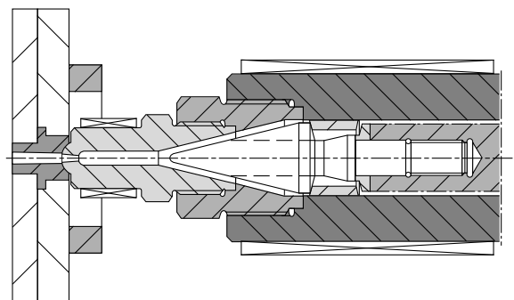
Fig. 22 Open nozzle adapter
