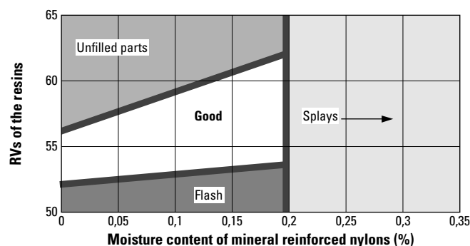
Fig. 13 Effect of RV and moisture content on the surface appearance of parts
