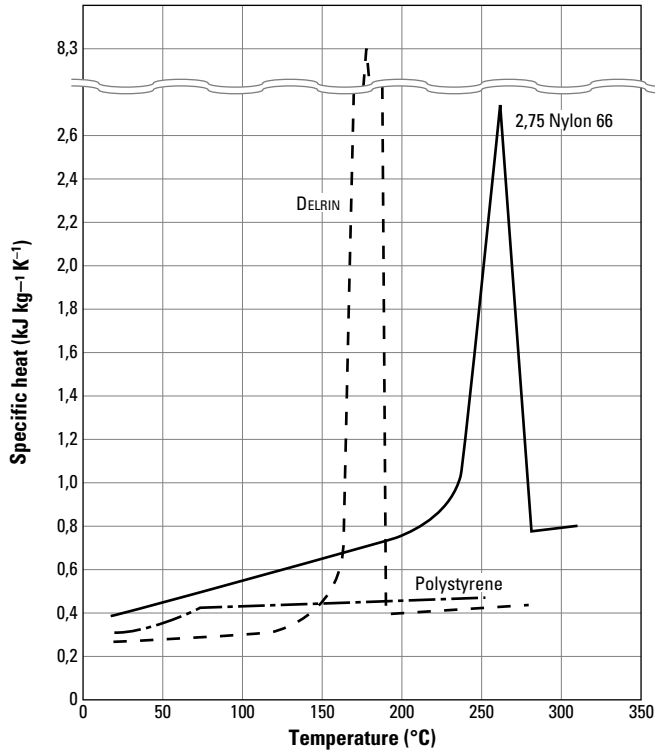
Fig. 2 Temperature dependence of specific heat
