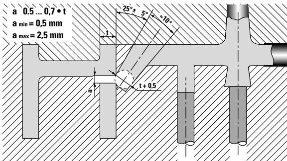
Fig. 24b Tunnel or submarine gate for unreinforced nylon
