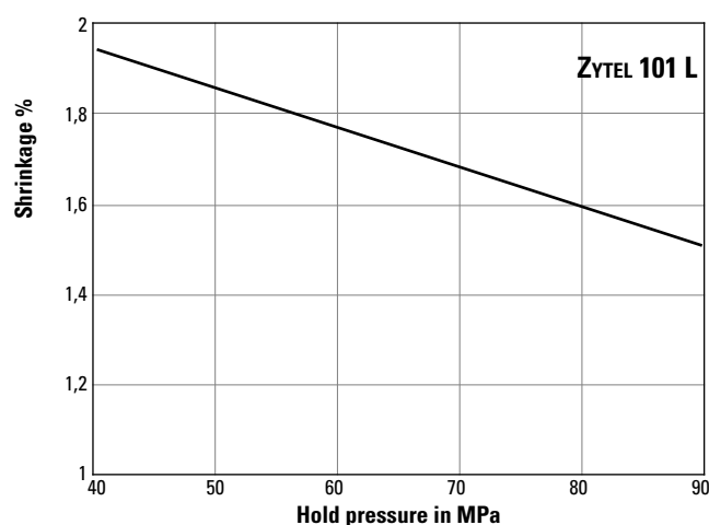
Fig. 44 Shrinkage as a function of hold pressure for a part 3 mm thick and a mould temperature of 70°C
