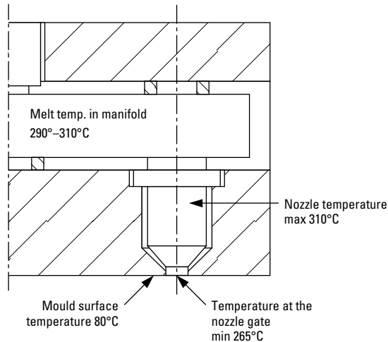
Fig. 28 Temperature in the hot runner area for PA 6.6
