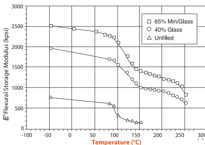
Figure 1 Flexural storage modulus vs. temperature for Fortron® PPS
