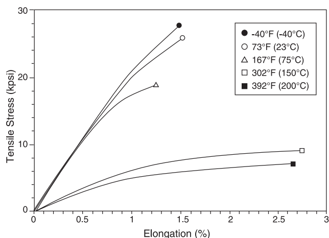
Figure 1 Stress-strain behavior of 40% glass-reinforced Fortron® PPS
