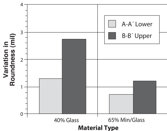
Figure 10 Warpage with respect to roundness of a cylinder
