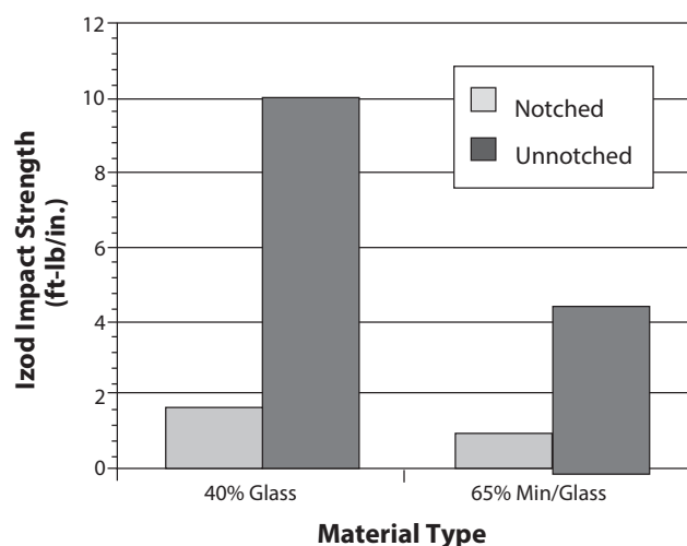
Figure 2 Effect of notches on Izod impact strength
