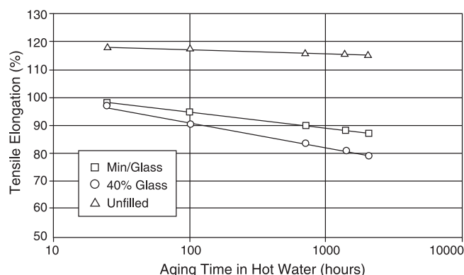
Figure 2 Tensile elongation in hot water under pressure
