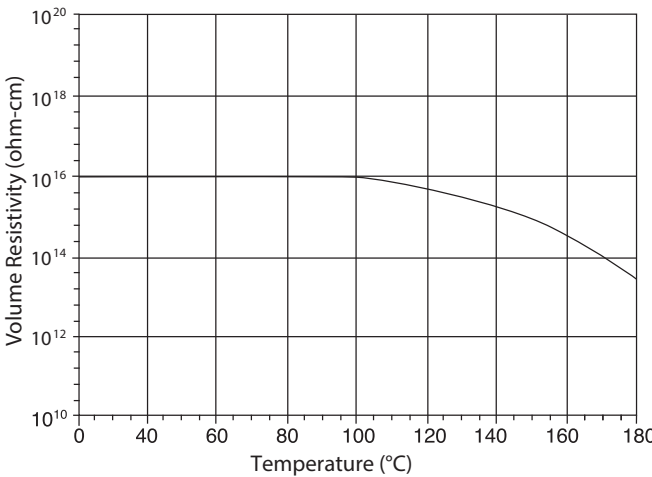
Figure 2 Effect of different temperatures on volume resistivity
