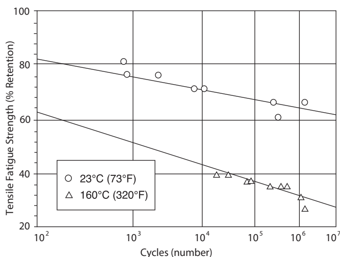
Figure 13 Fatigue resistance of 65% mineral/glass-reinforced Fortron® PPS
