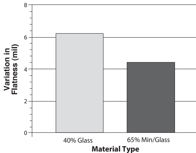
Figure 9 Warpage with respect to flatness
