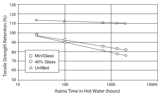
Figure 1 Tensile strength retention at break in hot water under pressure
