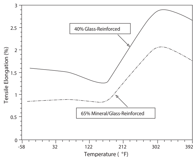
Figure 6 Temperature dependence of tensile elongation at break
