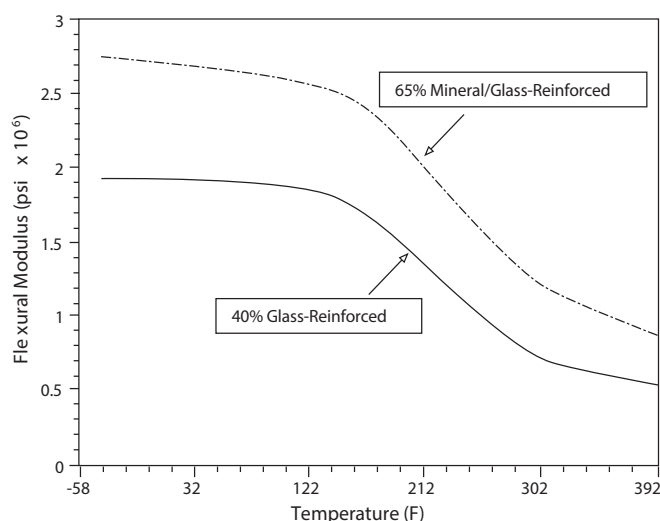
Figure 3 Temperature dependence of flexural strength
