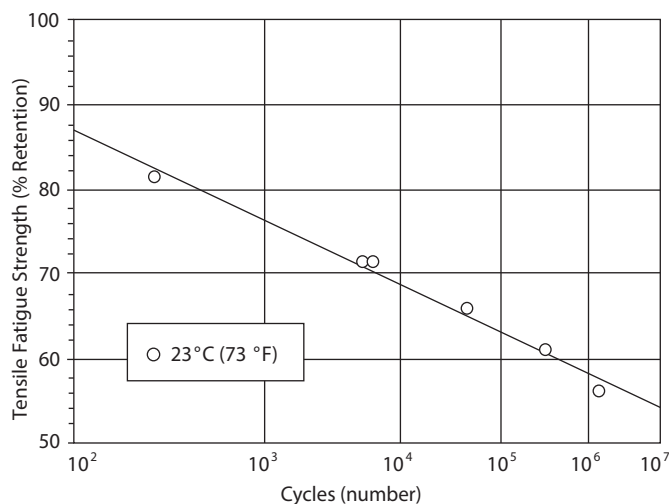
Figure 12 Fatigue resistance of 40% glass-reinforced Fortron® PPS
