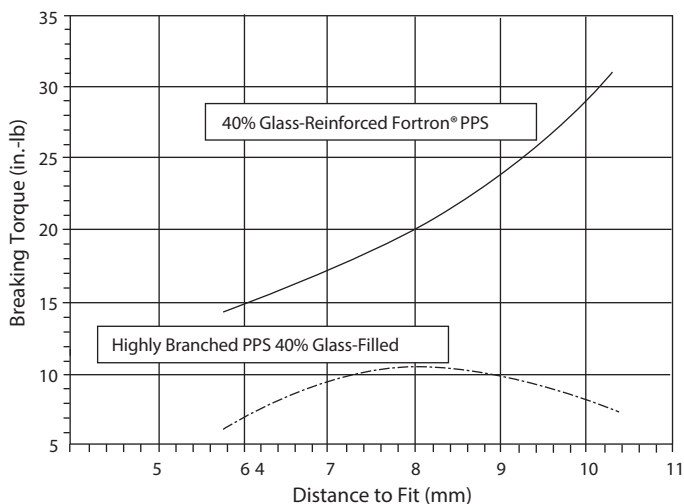
Figure 3 Breaking torque of a self-tapping screw
