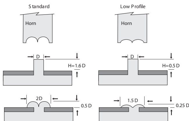
Figure 2 Dimensions for head forms for ultrasonic staking
