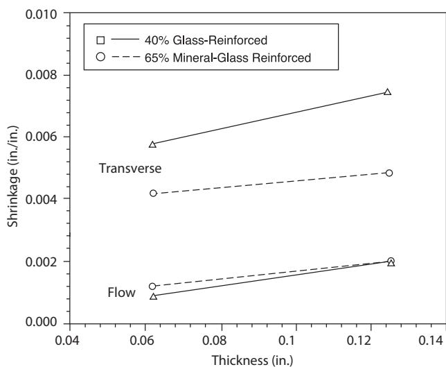
Figure 3 Effect of part thickness on shrinkage of Fortron® PPS
