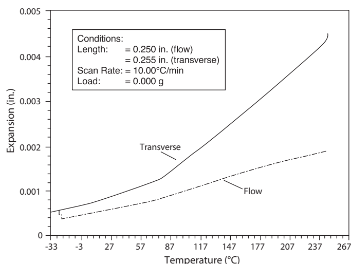
Figure 1 Dimensional change of mineral/glass-reinforced Fortron® PPS
