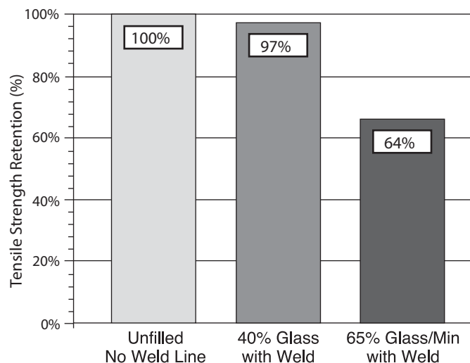
Figure 11 Weld line tensile strength vs. unfilled Fortron® PPS with no weld line
