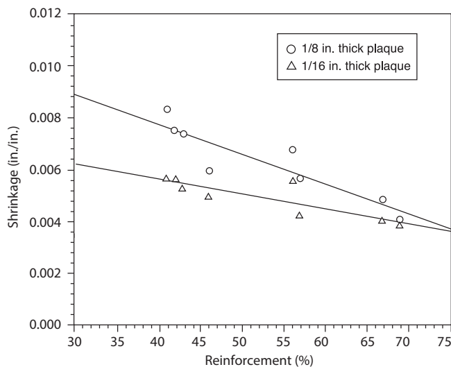
Figure 4 Effect of filler level on shrinkage of Fortron® PPS (Please note that not all reinforcement levels are available as commercial products.)
