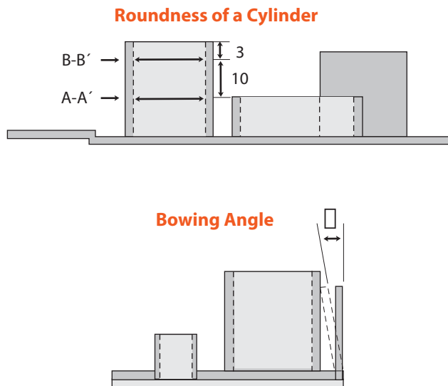
Figure 8 Measured points for warpage sample
