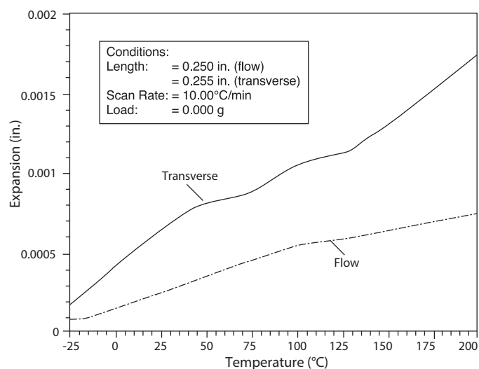
Figure 2 Dimensional change of 40% glass-reinforced Fortron® PPS
