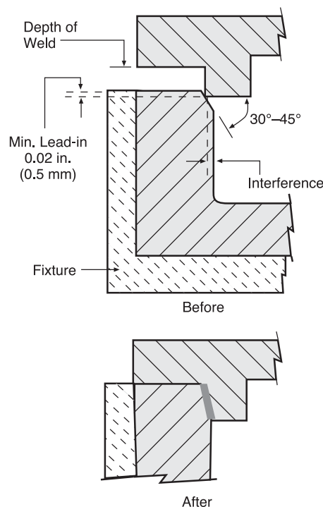
Figure 1 Recommended dimensions for shear joints
