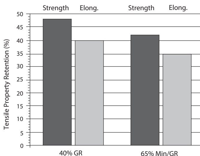
Figure 10 Comparison of tensile strength retention with and without weld lines
