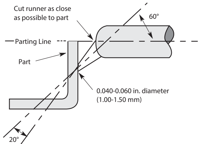
Figure 4 Specifications for submarine gates
