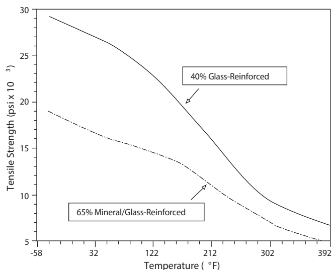
Figure 5 Temperature dependence of tensile strength at break
