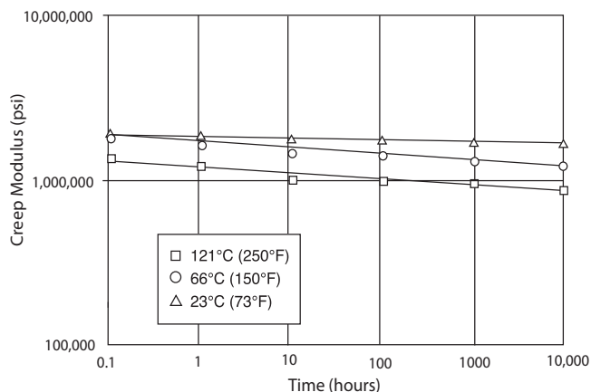
Figure 8 Creep modulus in three-point bending of 65% mineral/glass-reinforced Fortron® PPS; stress = 5000 psi
