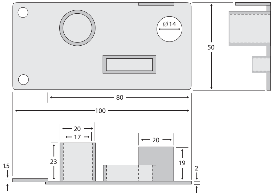
Figure 7 Specifications for warpage sample, dimensions in millimeters
