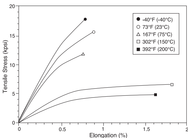
Figure 2 Stress-strain behavior of 65% mineral/glass-reinforced Fortron® PPS
