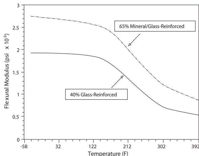
Figure 4 Temperature dependence of flexural modulus
