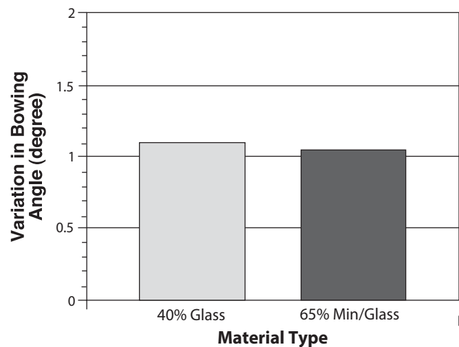
Figure 12 Warpage with respect to bowing angle
