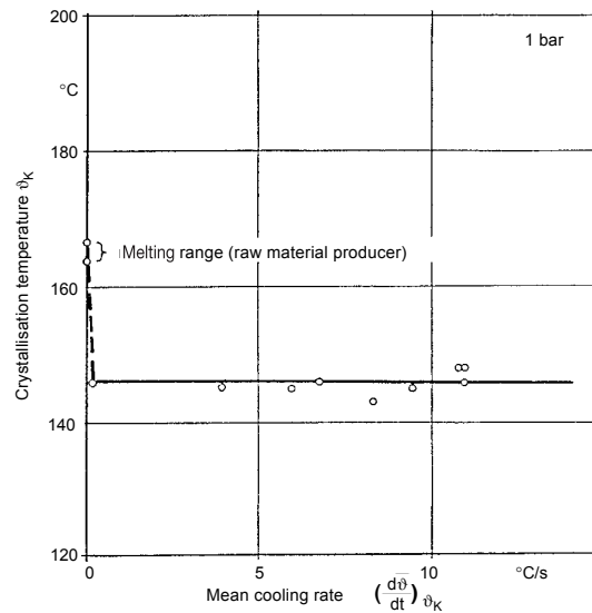
Fig. 11: Influence of cooling rate on crystallization temperature (Source: IKV)
