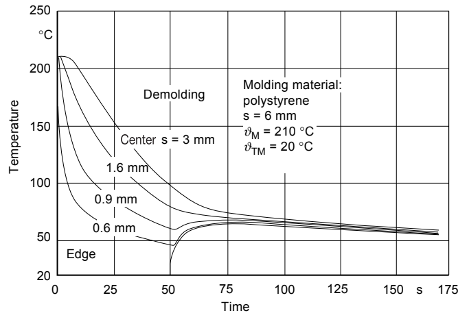
Fig. 20: Temperature profile in a plastics molding before and after demolding
