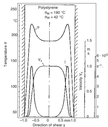
Fig. 1: Temperature profile in a flowing plastic melt [1]
