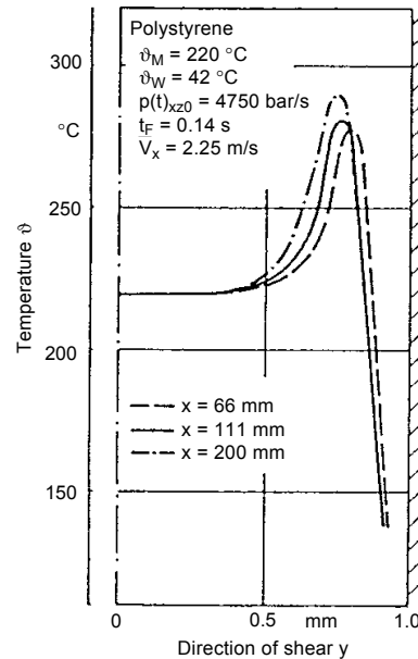
Fig. 2: Temperature profile at different flow locations at the time when the molded part is full [1]
