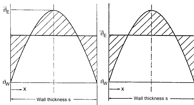
Fig. 15: Temperature profile in a thermoplastic molding at the time of demolding, demolding temperature \hat{\vartheta}_E in the center
