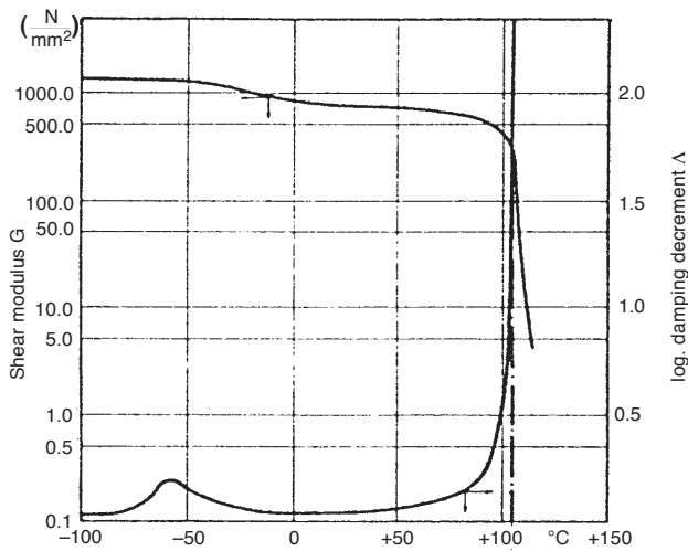
Fig. 18: Determination of the maximum demolding temperature from a shear modulus curve, material ABS
