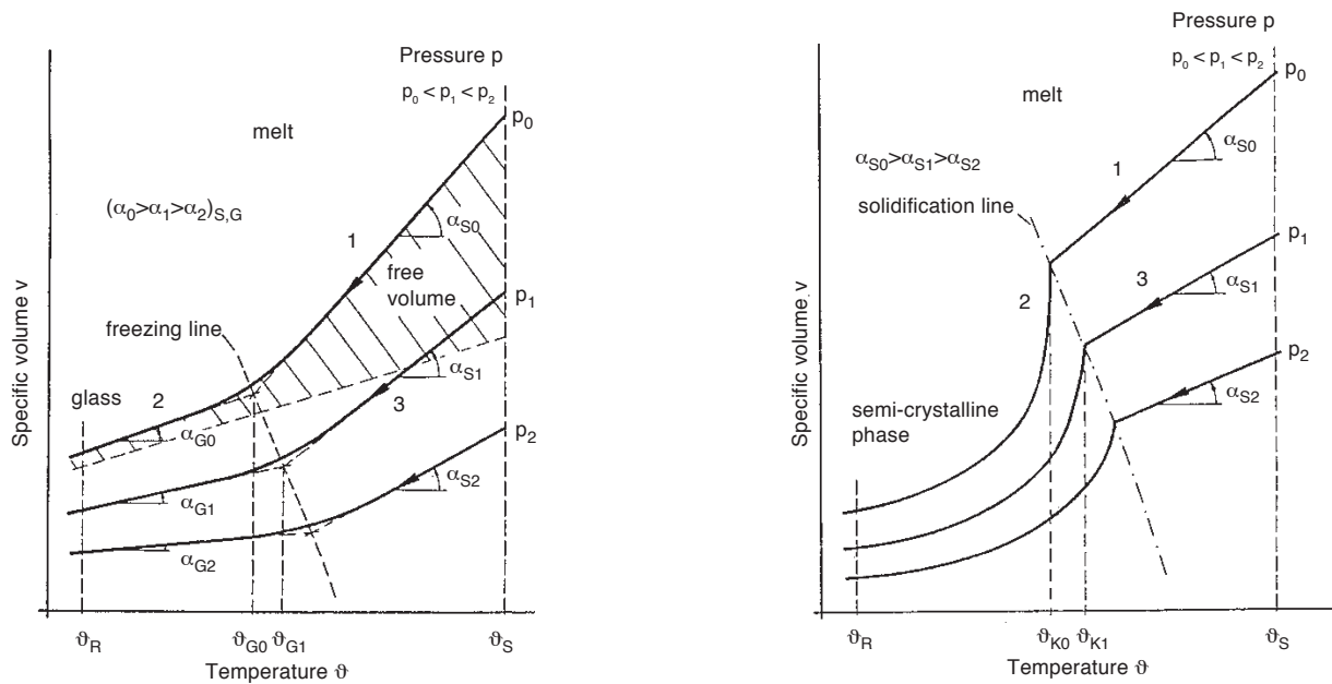
Fig. 6: p-v-θ-Diagram of a slowly cooling amorphous (left) and semi-crystalline (right) plastic (Source: IKV)
