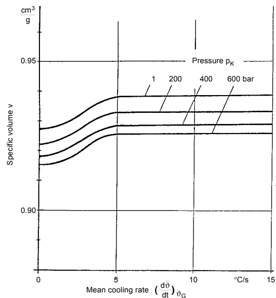
Fig. 8: Specific volume as a function of the cooling rate and pressure of an amorphous thermoplastic (Source: IKV)
