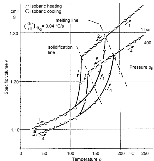
Fig. 10: Slow isobaric cooling and heating of a semi-crystalline thermoplastic (Source: IKV)
