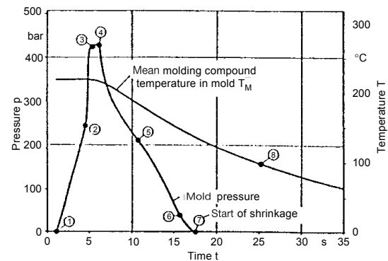
Fig. 12: Pressure and temperature profile during the injection molding cycle [4]
