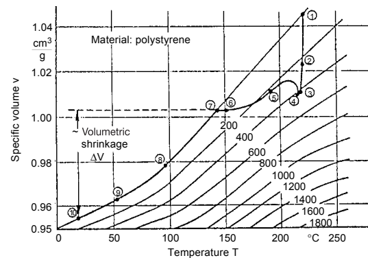
Fig. 13: State curve during injection molding [4]
