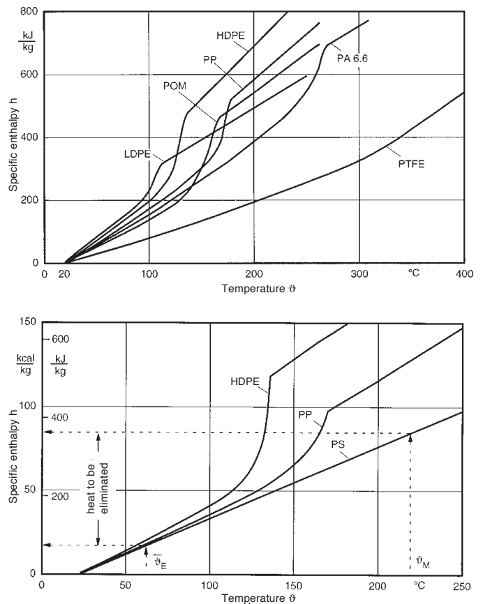
Fig. 22: Specific enthalpy as a function of temperature for a number of thermoplastics; p = 1 bar
