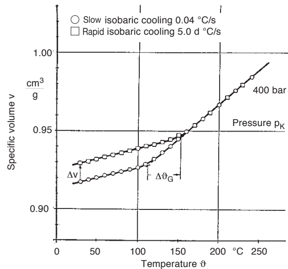
Fig. 7: Comparison of slow and rapid isobaric cooling of an amorphous thermoplastic (Source: IKV)
