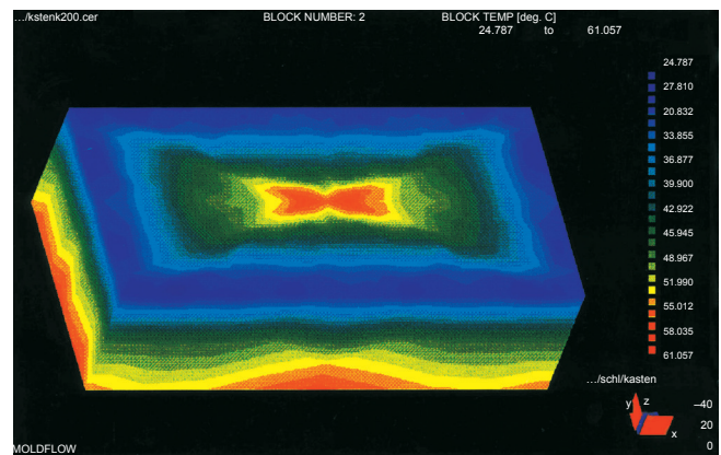
Fig. 21: Calculated mold surface temperature on the nozzle side of a box-shaped molded part
