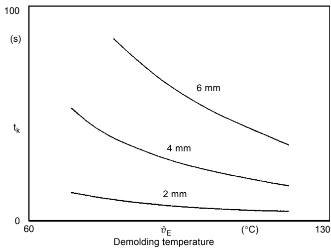
Fig. 14: Influence of demolding temperature on cooling time
