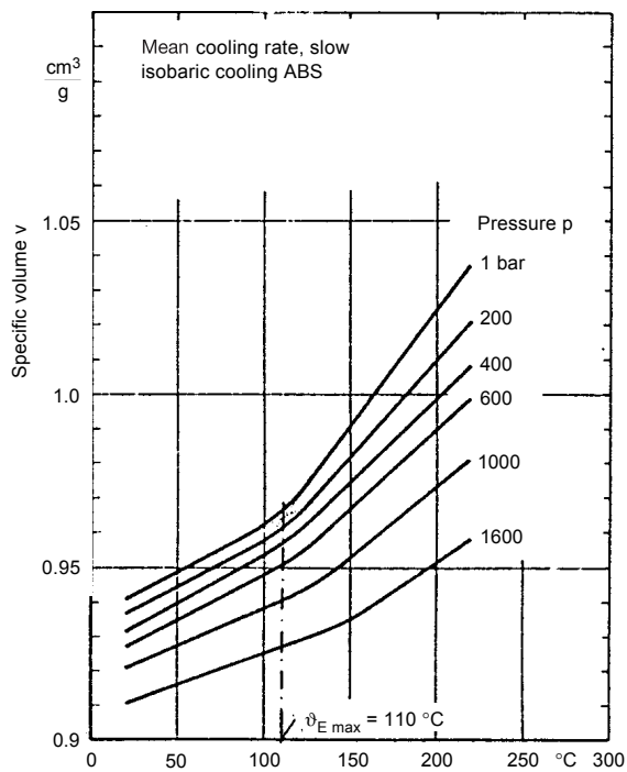
Fig. 19: Demolding temperature from the p-v-θ diagram, material ABS
