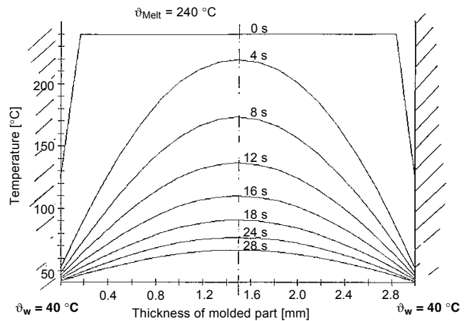
Fig 3: Temperature profiles in a cooling thermoplastic melt at different points in time (computed)
