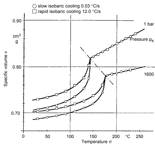
Fig. 9: Comparison of slow and rapid isobaric cooling of a semi-crystalline thermoplastic at two different pressures (Source: IKV)
