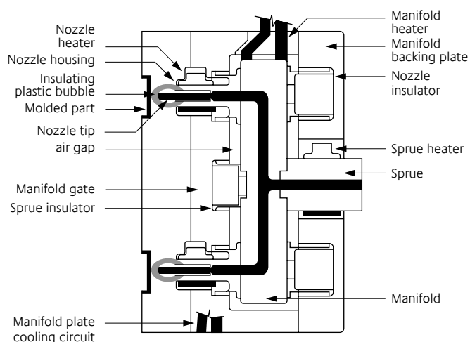
Figure 3 Hot runner manifold tool
