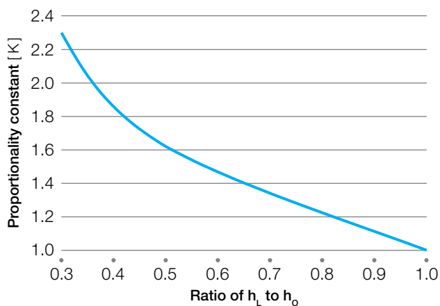
Figure 8.14 Proportionality constant (K) for tapered beam
