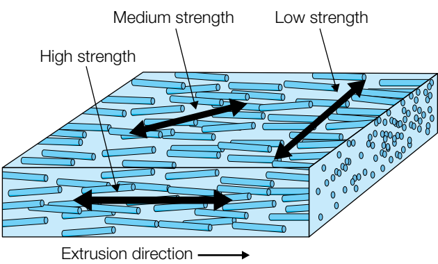
Figure 10.12 Fiber orientation affects strength
