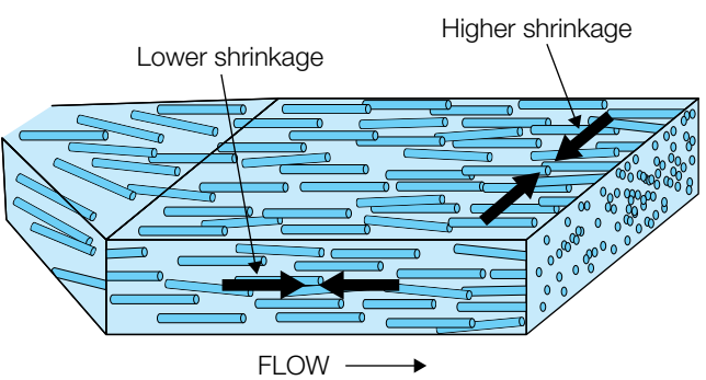
Figure 9.17 Shrinkage varies with flow direction
