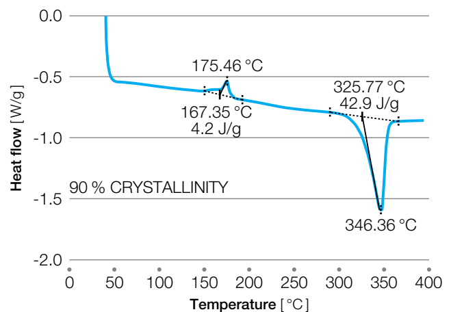
Figure 10.11 Sample DSC plot
