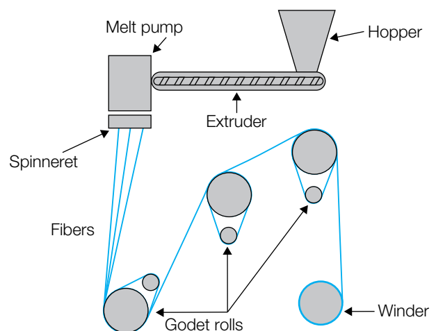
Figure 9.28 Fiber spinning process
