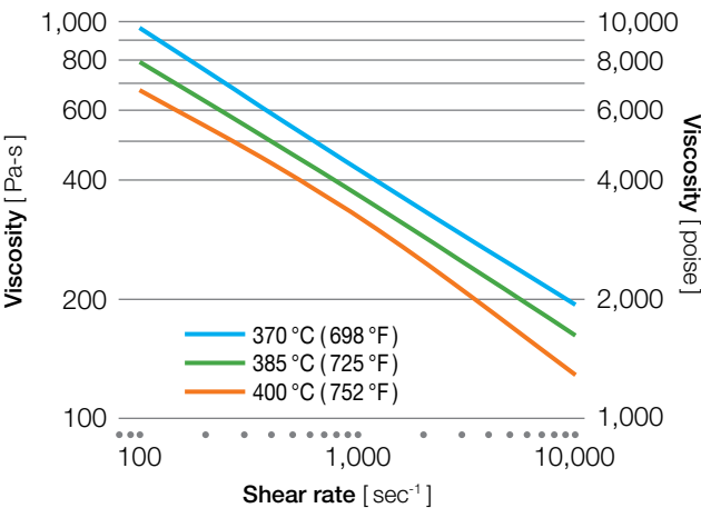
Figure 9.4 KetaSpire® KT-880 GF30
