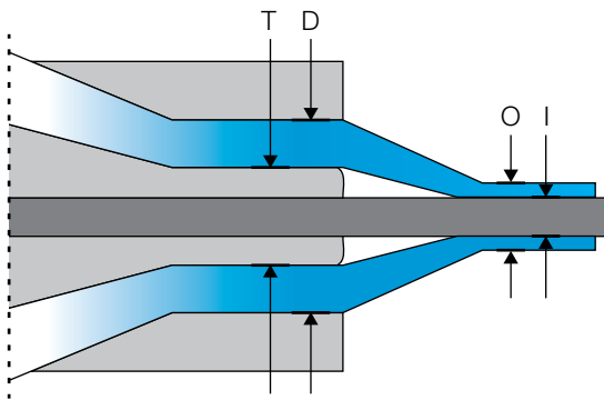
Figure 9.32 Sleeve die draw down ratio
