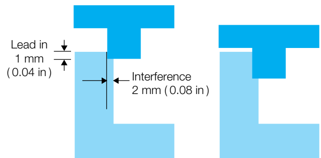
Figure 10.6 Shear joint
