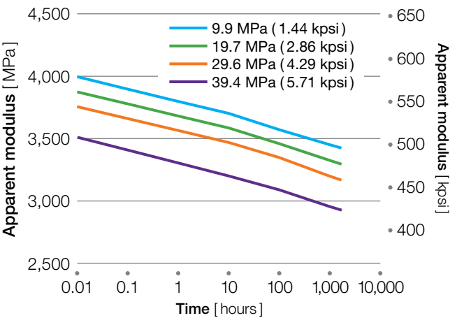
Figure 4.5 KT-820 NT at 23 °C (73 °F)
