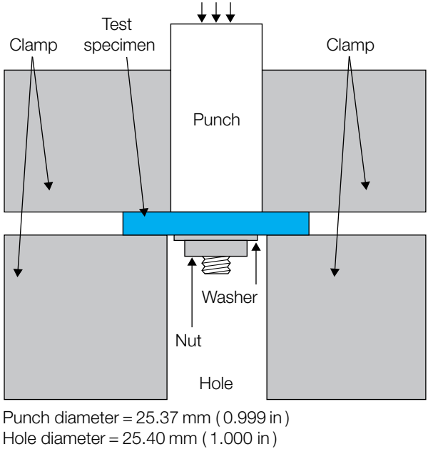
Figure 3.26 Diagram of shear test apparatus
