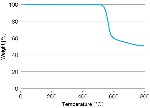
Figure 5.12 TGA KT-880 in N 2
