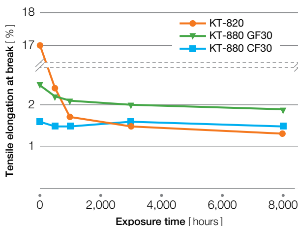
Figure 7.13 Tensile elongation at break
