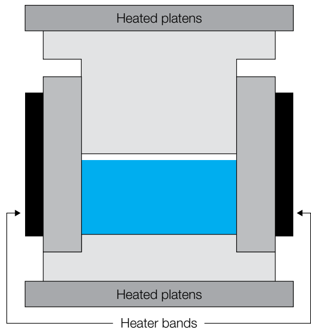
Figure 9.34 Tall molds need heater bands
