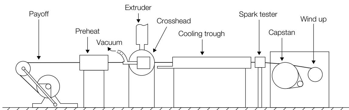
Figure 9.29 Typical wire extrusion equipment
