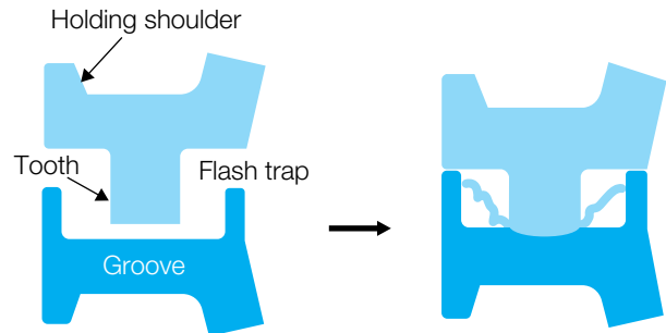
Figure 10.2 Typical vibrational welding joint
