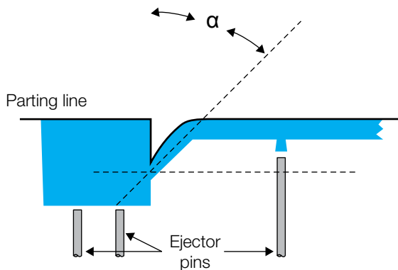
Figure 9.19 Tunnel gate
