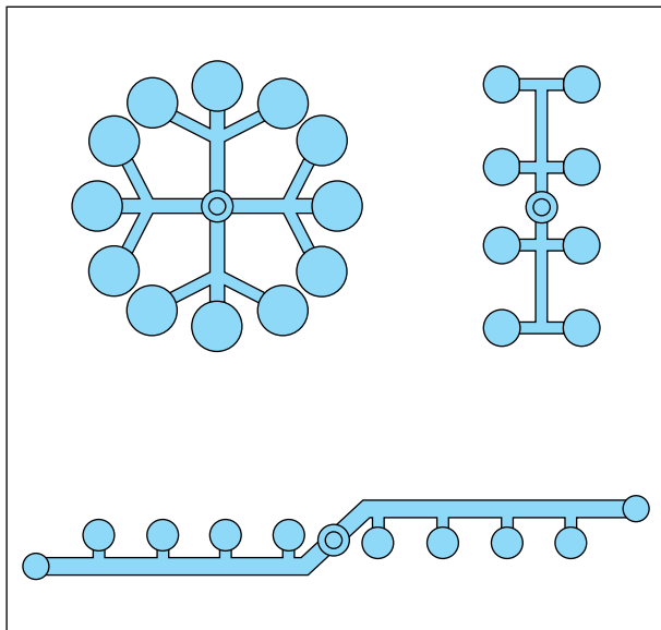
Figure 9.15 Balanced
