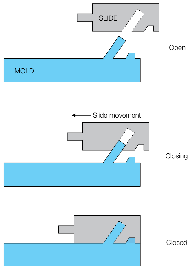
Figure 9.16 Angled pin slide schematic
