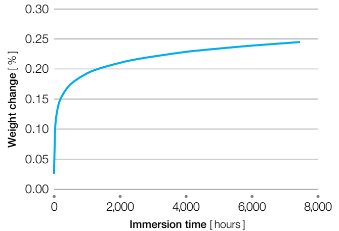
Figure 7.15 Water absorption of KetaSpire® KT-820 GF30
