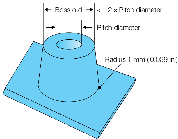
Figure 8.8 Boss design for self-tapping screws
