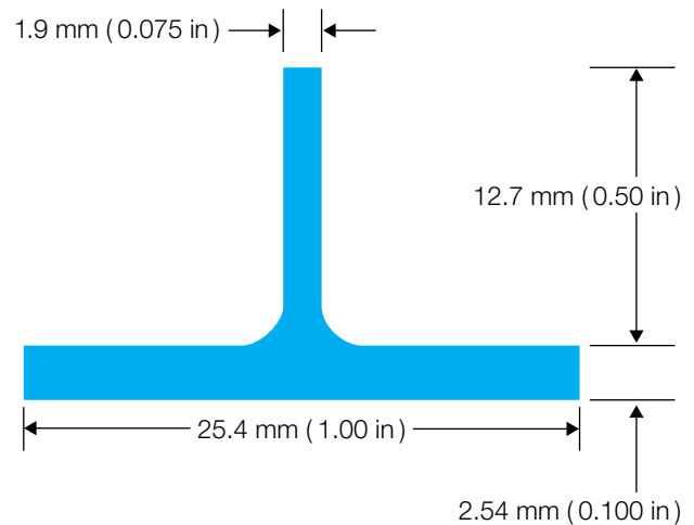
Figure 8.5 Rib design example
