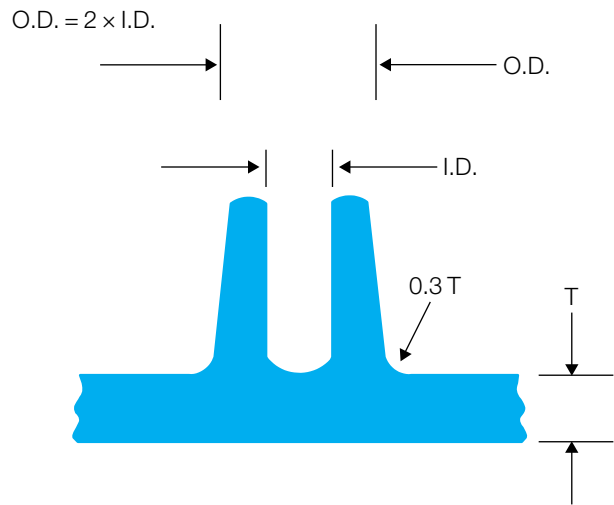
Figure 8.18 Boss design - general guidelines
