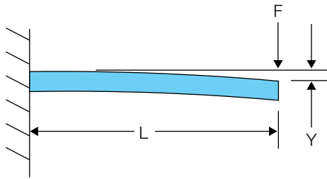
Figure 8.12 Cantilever beam - concentrated load at free end
