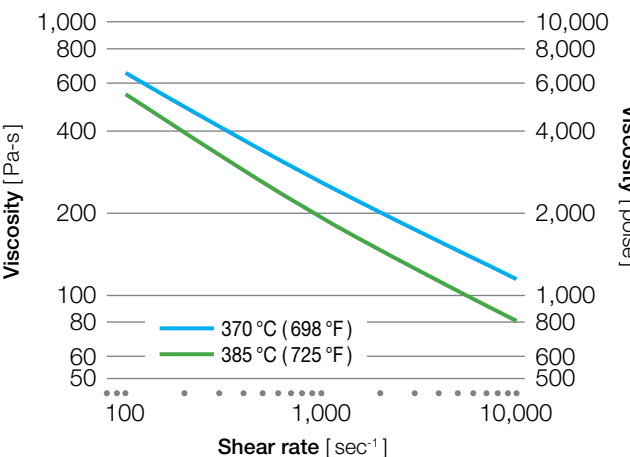
Figure 9.7 KetaSpire® KT-820 SL10
