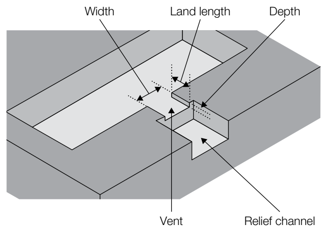
Figure 9.20 Vents
