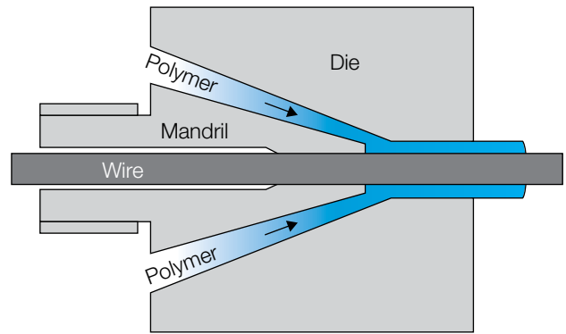
Figure 9.30 Schematic of pressure die
