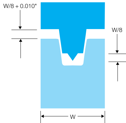
Figure 10.6 Shear joint
