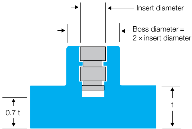
Figure 8.10 Boss design for ultrasonic inserts
