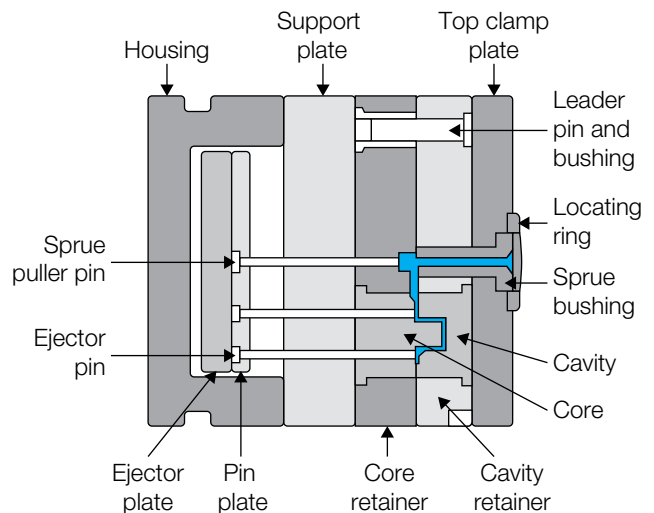
Figure 9.12 Two plate tool
