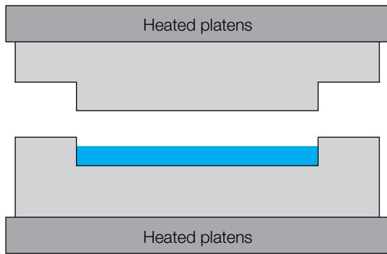
Figure 9.35 Short flat molds can use platen heat
