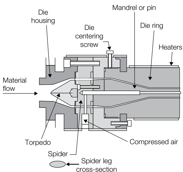
Figure 9.26 Tubing die
