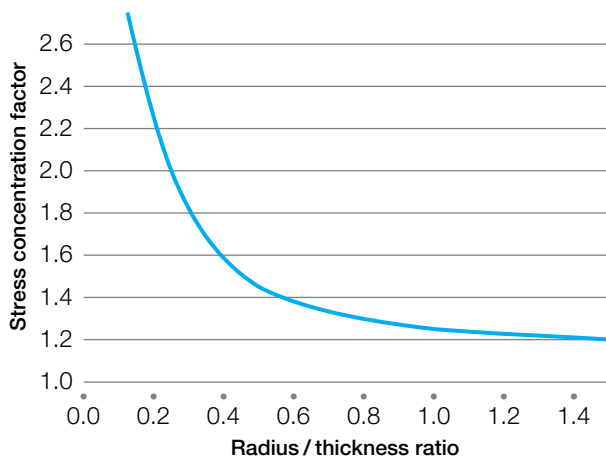
Figure 8.6 Stress concentration at inside corners
