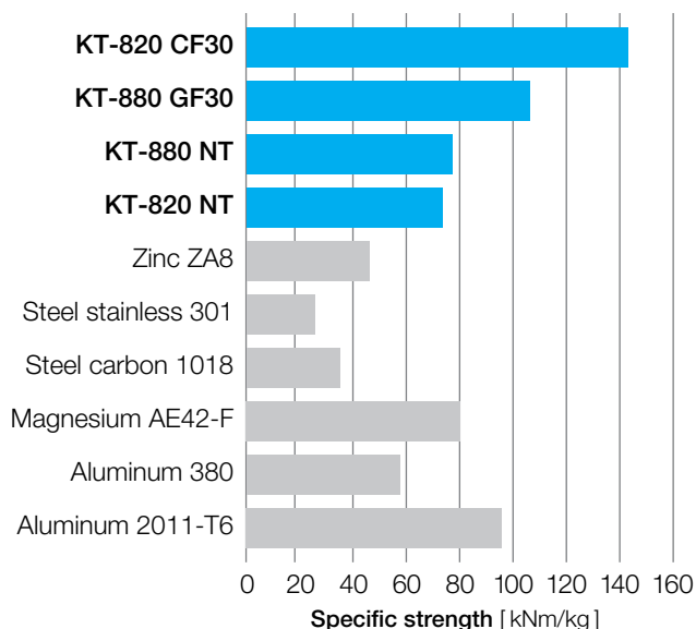
Figure 8.1 Specific strength
