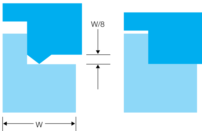
Figure 10.4 Step joint
