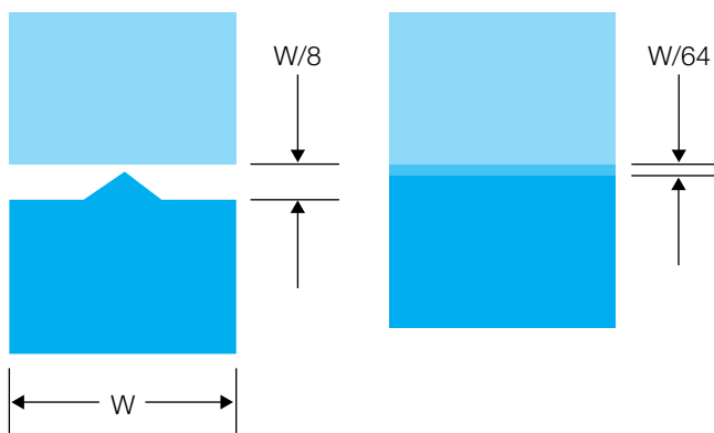
Figure 10.4 Step joint
