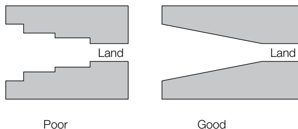
Figure 9.23 Adapter design
