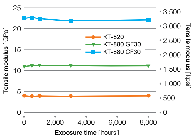
Figure 7.12 Tensile modulus
