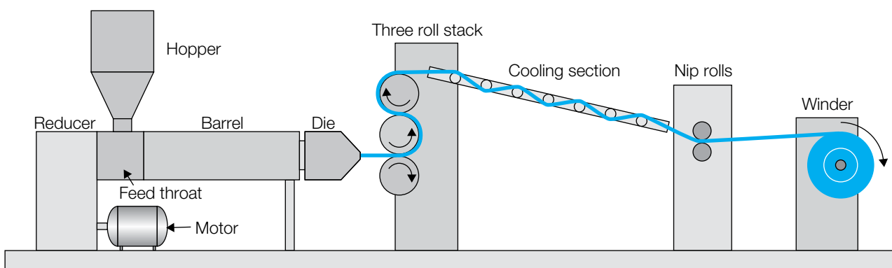
Figure 9.25 Typical three-roll stack
