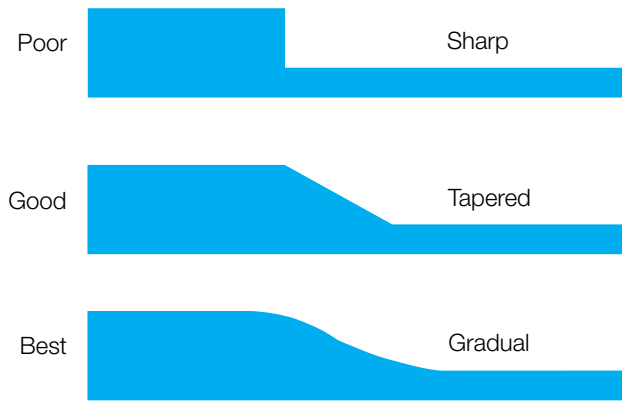
Figure 8.16 Draft - designing for mold release
