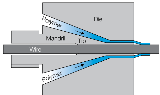
Figure 9.31 Schematic of sleeve die
