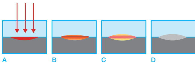
Figure 10.7 Laser welding process
