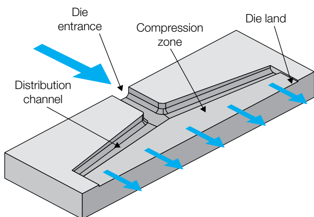
Figure 9.24 Coat hanger film die conceptual lower die plate
