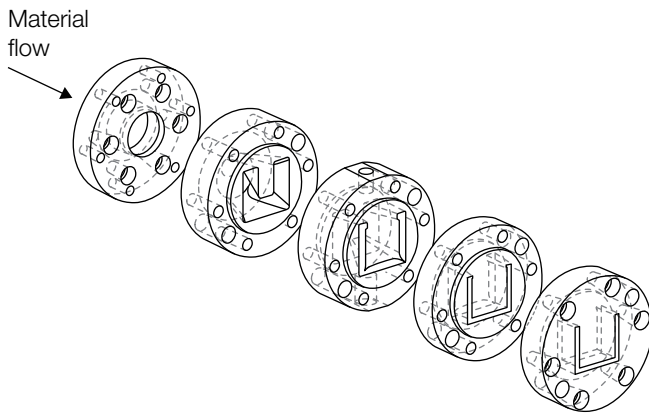
Figure 9.27 Typical profile extrusion die
