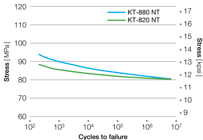
Figure 4.13 Fatigue of carbon fiber reinforced KetaSpire® PEEK at 23 °C (73 °F)
