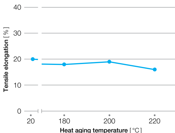
Figure 5.7 Tensile elongation after 8,000 hours
