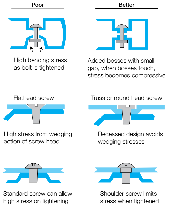
Figure 8.7 Designing for mechanical fasteners
