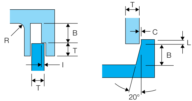
Figure 10.1 Typical spin weld joint designs
