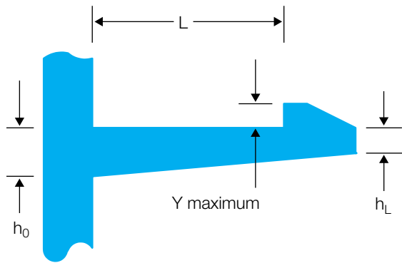
Figure 8.13 Snap fit design using tapered beam
