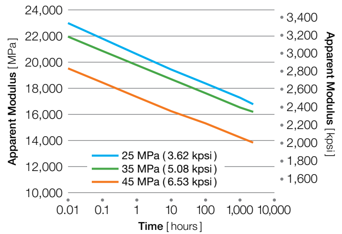
Figure 4.10 KT-820 CF30 at 160 °C (320 °F)
