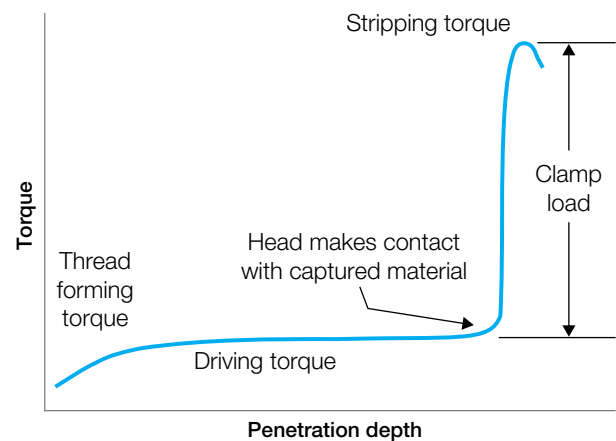
Figure 8.9 Torque developed during screw installation
