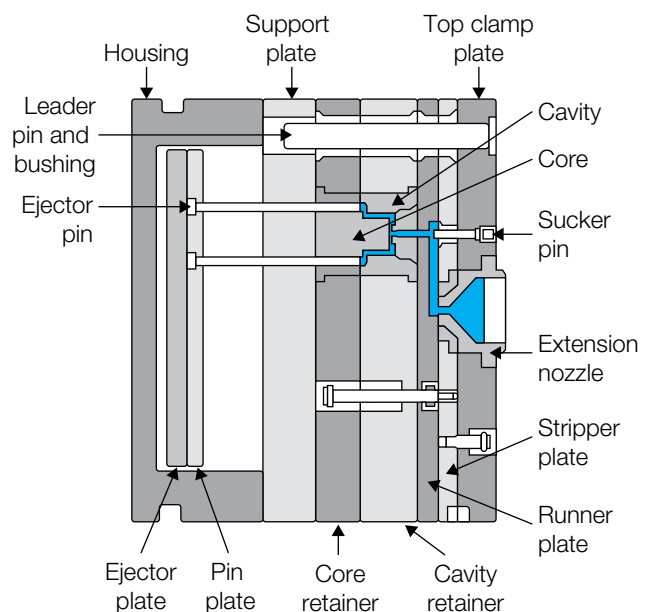
Figure 9.13 Three plate tool
