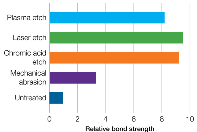
Figure 10.8 Surface preparation and bond strength
