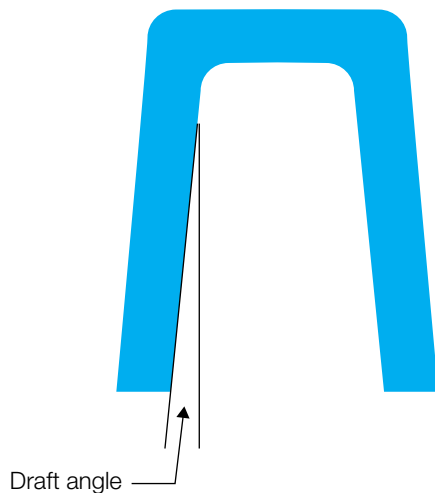
Figure 8.17 Draft - recommended rib design
