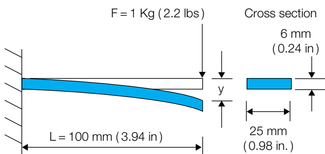
Figure 8.4 Beam used for examples
