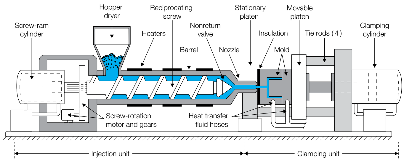
Figure 9.10 Injection molding machine schematic
